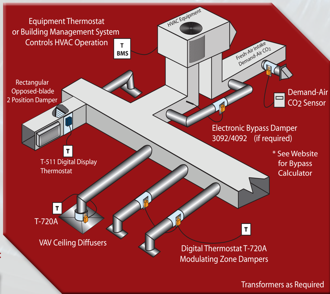
T-511 Digital Thermostat
